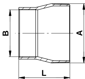
Fig. 29 Dimensional sketch and photo of the connecting piece thread-to-thread
