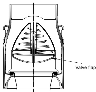
Fig. 5 Non-return valve
