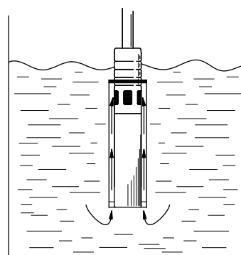
Fig. 32 Flow sleeve function
